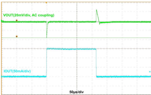
Figure 18. LDO1/2 Load Transient, V_{IN} = 3.8\text{ V} , V_{OUT} = 2.85\text{ V} , 1 mA \leftrightarrow 150 mA, 1 \mu\text{s} Edge
