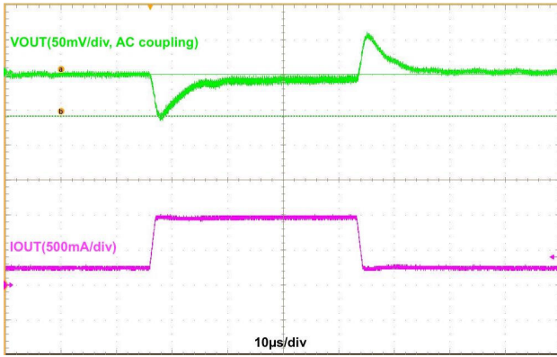
Figure 16. Buck Load Transient, V_{IN} = 3.8\text{ V} , V_{OUT} = 1.1\text{ V} , 240 mA \leftrightarrow 960 mA, 1 \mu\text{s} Edge, Auto Mode
