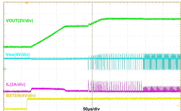
Figure 21. Boost Start-up, V_{IN} = 3.8\text{ V} , V_{OUT} = 5.0\text{ V} , 100 mA Resistive Load, Auto Mode
