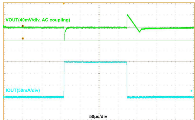
Figure 19. LDO3/4 Load Transient, V_{IN} = 1.95\text{ V} , V_{OUT} = 1.8\text{ V} , 1 mA \leftrightarrow 150 mA, 1 \mu\text{s} Edge
