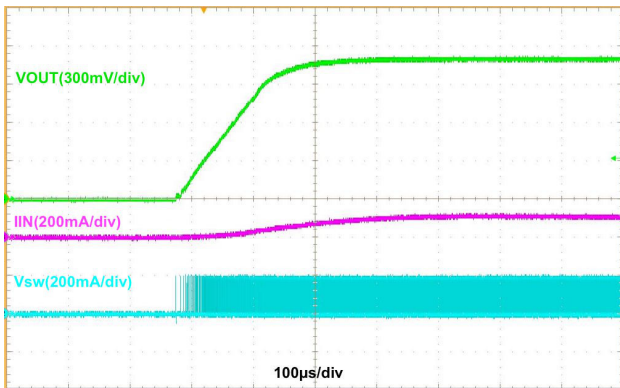
Figure 20. Buck Start-up, V_{IN} = 3.8\text{ V} , V_{OUT} = 1.1\text{ V} , 300 mA Resistive Load, Auto Mode
