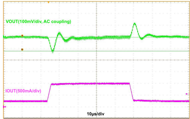
Figure 17. Boost Load Transient, V_{IN} = 3.8\text{ V} , V_{OUT} = 5.0\text{ V} , 200 mA \leftrightarrow 800 mA, 2 \mu\text{s} Edge, Auto Mode
