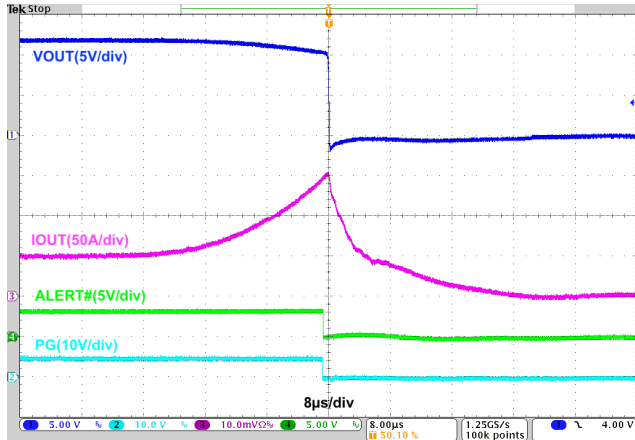
Figure 22. Short Circuit During Normal Operation, Initial IOU = 50 A
