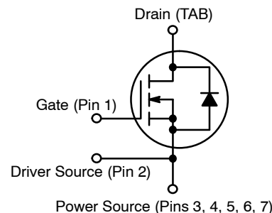
N-CHANNEL MOSFET
