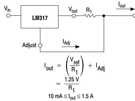
Figure 26. Current Regulator
