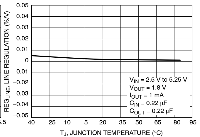
Figure 8. Line Regulation vs. Temperature V OUT = 1.8 V
