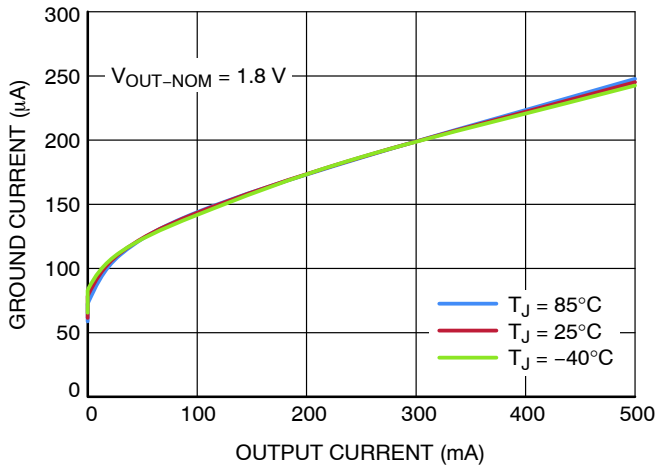
Figure 15. Ground Current vs. Output Current
