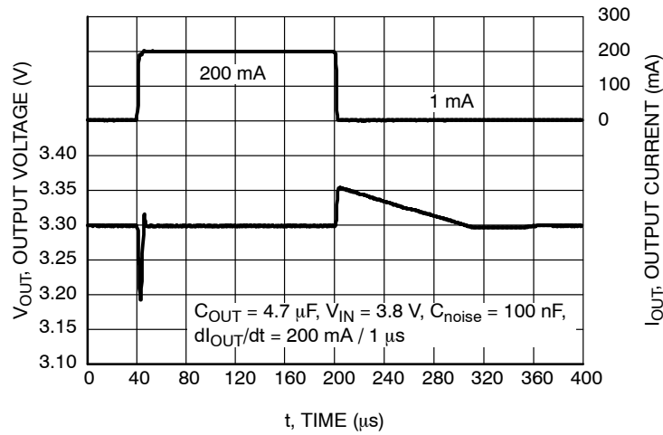
Figure 28. Load Transient Response, V OUT = 3.3 V, C OUT = 4.7 μF, C noise = 100 nF
