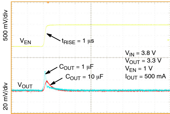
Figure 50. Line Transient Response – Rising Edge, V_{OUT} = 3.3\text{ V} , I_{OUT} = 500\text{ mA}
