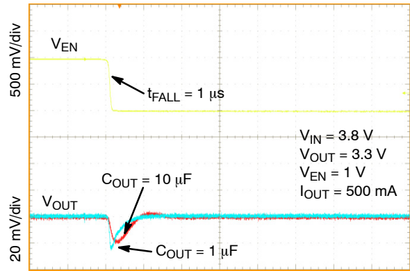
Figure 51. Line Transient Response – Falling Edge, V_{OUT} = 3.3\text{ V} , I_{OUT} = 500\text{ mA}
