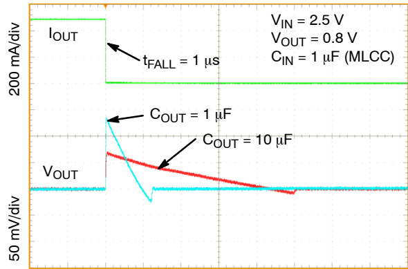
Figure 53. Load Transient Response – Falling Edge, V_{OUT} = 0.8\text{ V} , I_{OUT} = 1\text{ mA} to 500\text{ mA} , C_{OUT} = 1\text{ μF} , 10\text{ μF}
