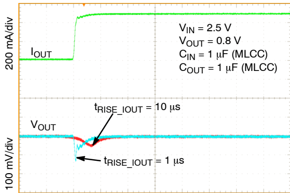
Figure 54. Load Transient Response – Rising Edge, V_{OUT} = 0.8\text{ V} , I_{OUT} = 1\text{ mA} to 500\text{ mA} , t_{RISE\_IOUT} = 1\text{ μs} , 10\text{ μs}
