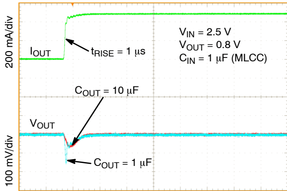
Figure 52. Load Transient Response – Rising Edge, V_{OUT} = 0.8\text{ V} , I_{OUT} = 1\text{ mA} to 500\text{ mA} , C_{OUT} = 1\text{ μF} , 10\text{ μF}
