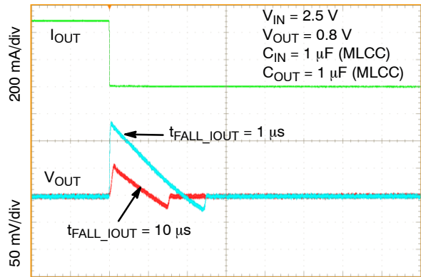
Figure 55. Load Transient Response – Falling Edge, V_{OUT} = 0.8\text{ V} , I_{OUT} = 1\text{ mA} to 500\text{ mA} , t_{FALL\_IOUT} = 1\text{ μs} , 10\text{ μs}
