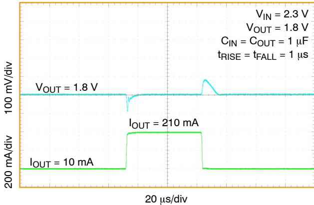
Figure 13. Load Transient Response, 10 mA – 210 mA NCV8752A/B, V_{OUT} = 1.8\text{ V}
