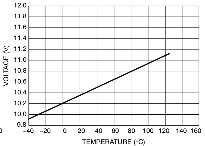
Figure 18. 8P5 Output Clamp vs. Temperature
